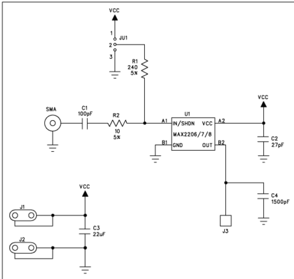
Figure 3. The MAX2208 evaluation kit schematic
