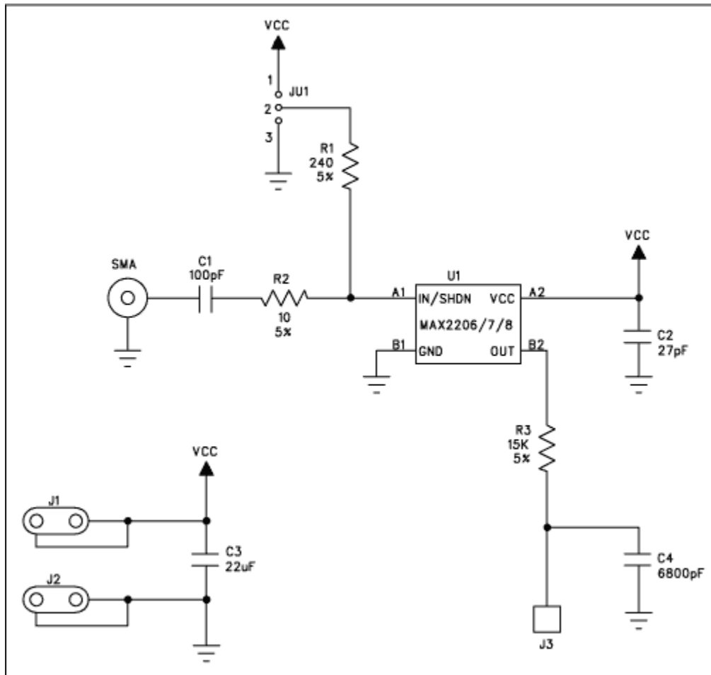
Figure 4. The MAX2206 evaluation kit schematic
